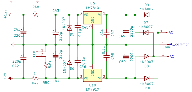
Limiter with M5283P VCA chip
